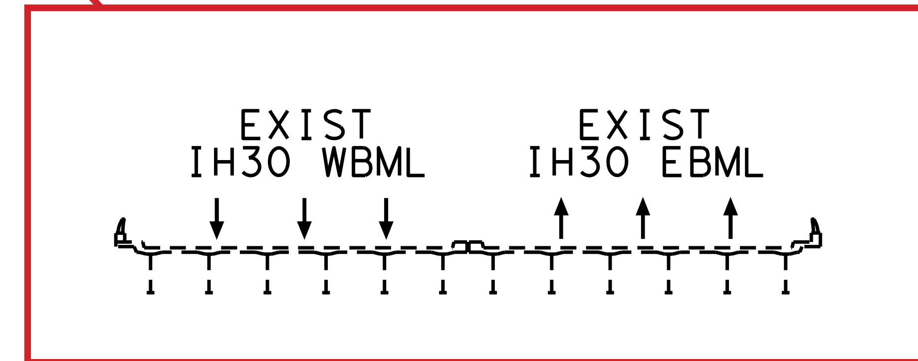
EXISTING I-30 BEFORE RECONSTRUCTION
